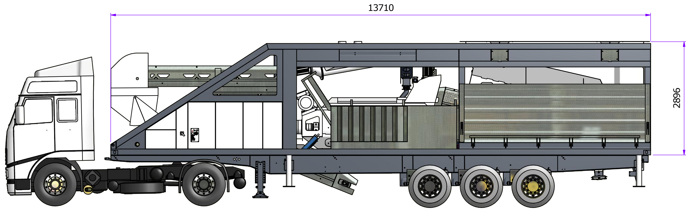
Mixer trailer
