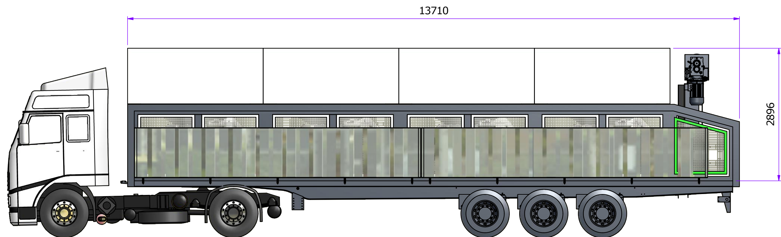
Aggregates trailer
